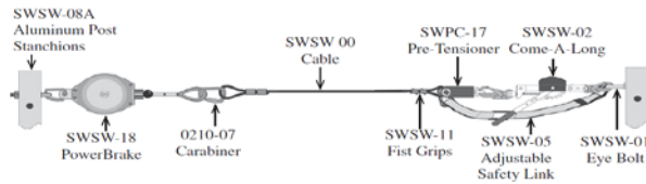
Sample diagram of SWSW Series Mobile SkyWalk horizontal lifeline system. Not all components are reflected in this diagram.
