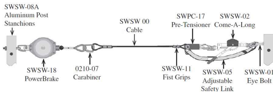
Sample diagram of SWSW Series Mobile SkyWalk horizontal lifeline system. Not all components are reflected in this diagram.
